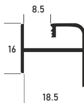
HORIZONTAL CENTRAL FOR GLASS
