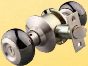
CN5127 BN/US32D 60/70BS Cylindrical Knobset- Entrance, 65mm Rose, 60/70mm B/S (SSS)
