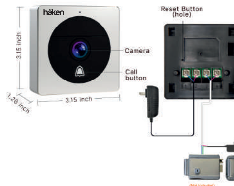
Main Unit
